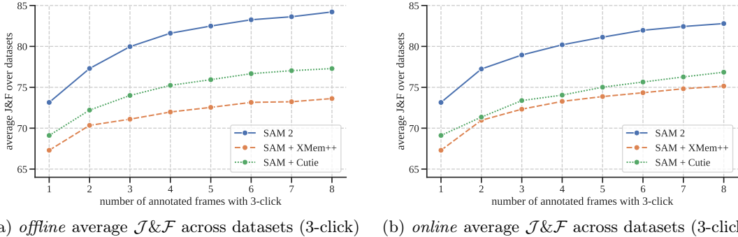
Figure 6 Zero-shot accuracy over 9 datasets in interactive offline and online evaluation settings.
