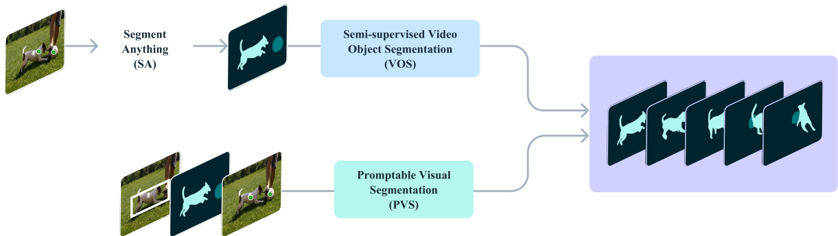
Figure 8 An illustration of the Promptable Visual Segmentation task (PVS). Previously studied tasks such as Segment Anything (SA) and semi-supervised Video Object Segmentation (VOS) can be seen as special cases of the PVS task.
