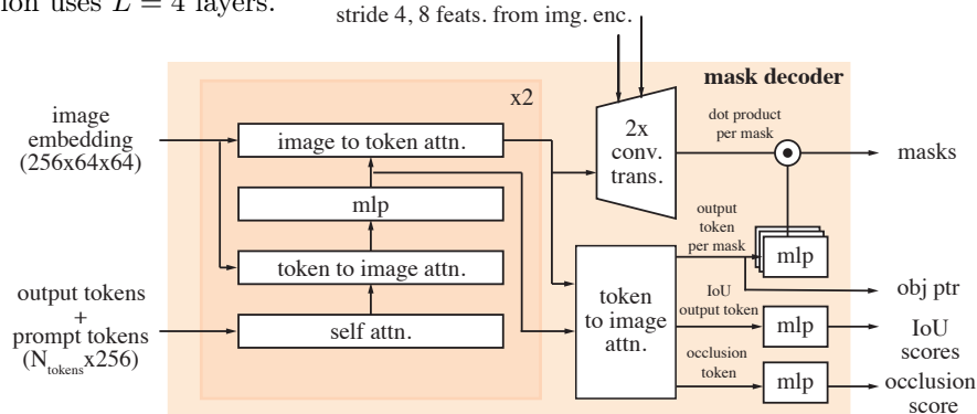
Figure 9 Mask decoder architecture. The design largely follows SAM, and we additionally include the stride 4 and 8 features from the image encoder during upsampling. We also use the mask token corresponding to the output mask as an object pointer and generate an occlusion score which indicates if the object of interest is visible in the current frame.
