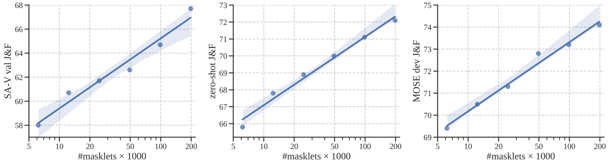
Figure 7 Performance of SAM 2 as a function of the SA-V quantity. We report \mathcal{J}\&\mathcal{F} accuracy for 3-click prompts in the first frame on SA-V val (left), 9 zero-shot datasets (center), and MOSE dev (right).
