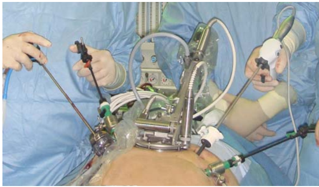
Figure 1: VikY Robot
