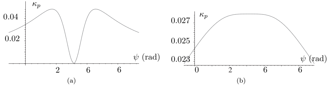
Figure 10: Pitch-curve curvature for p = 50 mm: (a) \eta = 1/\pi and (b) \eta = 2/\pi
