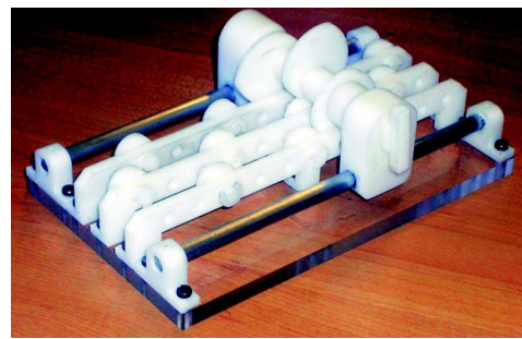
Figure 15: Layout of the three conjugate-cam mechanism on the same shaft
