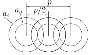
Figure 12: Geometric constraint on the roller-pin radius
