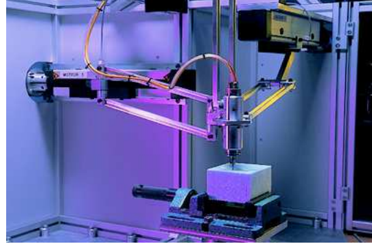
Figure 2: The Orthoglide
