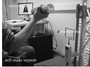
Fig. 1 Measurement device
