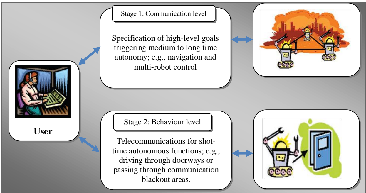
Fig. 1. Mobile robots - two levels of information procession. Communication concerns the high level within the whole group. Behaviour (behavioural level) – mean local decision making network.
