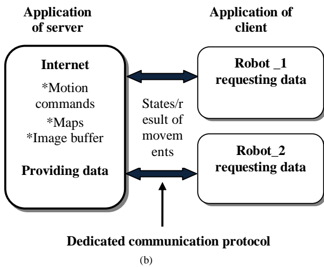
Fig. 4. General concept of internet architecture: communication medium between client (Internet) and server (Robot) – a, communication medium between server (Internet) and client (Robot) – b [46].
