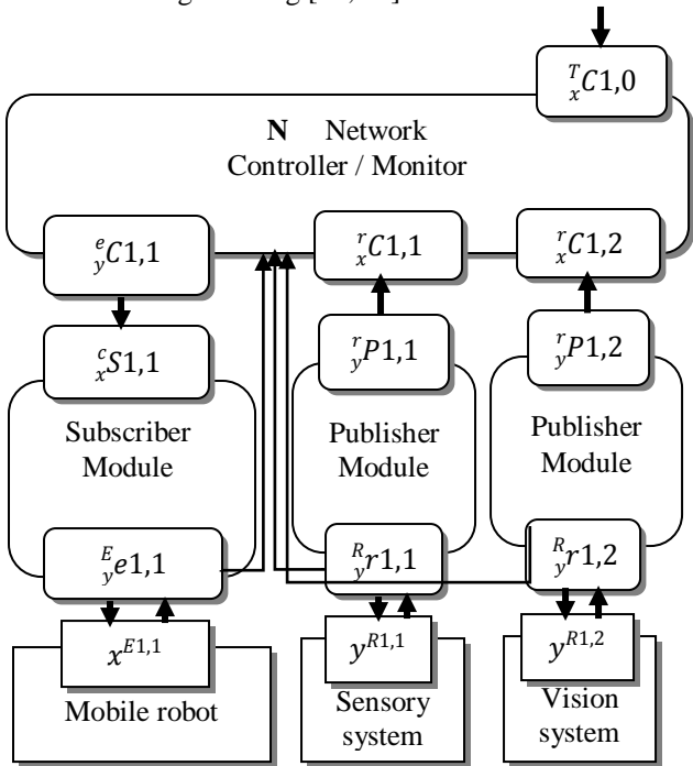
Fig. 3. Shows the structure of mobile robot- Internet interface proposed using the concept proposed in [42, 28] and adapted in [31].
